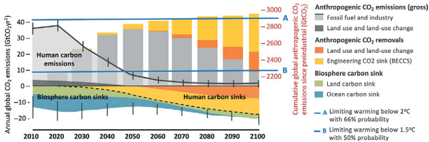
FIGURE 16.5 Cumulative and annual emissions and sinks of \text{CO}_2 are shown for stabilizing global climate at below 2^\circ\text{C} and 1.5^\circ\text{C} . Most of the carbon emissions shown in gray are energy-related. Together with land-use emissions they need to decline toward zero by midcentury. The figure is called Carbon Law as a metaphor to Moore's Law of semiconductors, where a number of transistors on a chip doubled every two and a half years. Carbon Law indicates that global emissions need to be halved every decade. In addition, human carbon sinks need to increase to almost half the magnitude of current positive emissions: This is a tall order. Carbon capture from biomass (bio-energy use with carbon capture and storage – BECCS) and land-use change are here the key. Third, biosphere carbon sinks need to be maintained as atmospheric concentrations decline. The vertical gray bars show cumulative emissions since the beginning of the industrial revolution of some 2,000 billion tons \text{CO}_2 . This budget, or carbon endowment of humanity, will be exhausted shortly as the remaining emissions for achieving stabilization at below 1.5^\circ\text{C} are essentially nil while we still emit some 40 billion tons \text{CO}_2 per year. Net-negative emissions are needed to stay within this budget. The remaining budget for stabilizing at 2^\circ\text{C} is a bit more generous so that the demand on net-negative emissions can be significantly reduced. The Carbon Law can be seen as a roadmap toward making the Paris Agreement and the SDGs a reality. Pathways shown in this report such as the SSP1 variant focused at the 1.5^\circ\text{C} target or the alternative scenarios portray similar dynamics, whereas the latter is unique among stabilization pathways as it does not need net negative emissions because of vigorous changes in end-use technologies and behaviors. (Source: Rockström et al. (2017); Figure published by TWI 2050 under CC-BY-NC 4.0)
